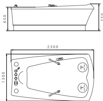
Maße California Twin
